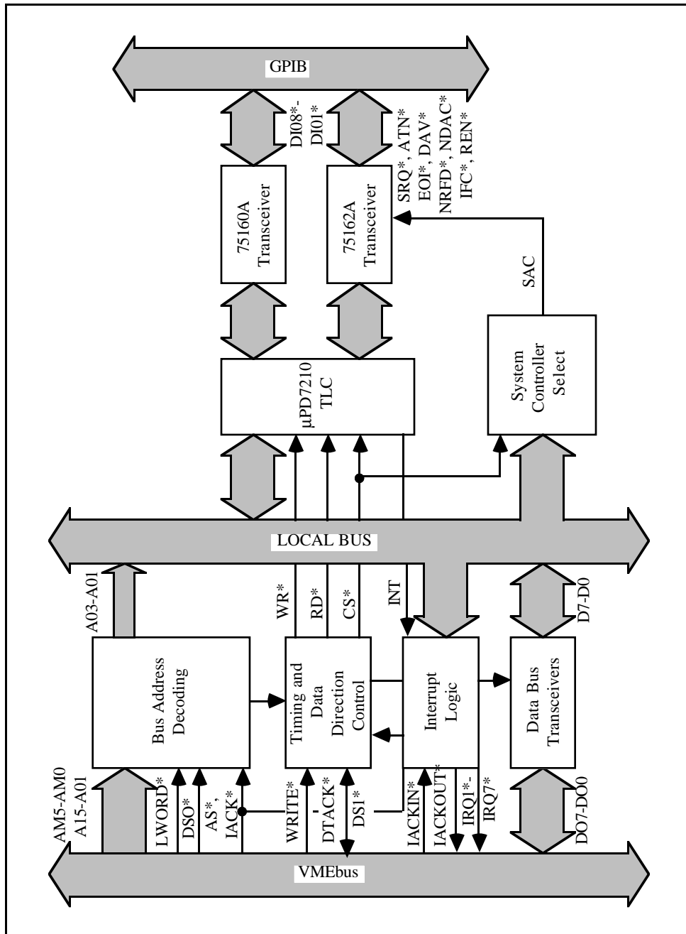
Figure 2-3. GPIB-1014P Block Diagram
