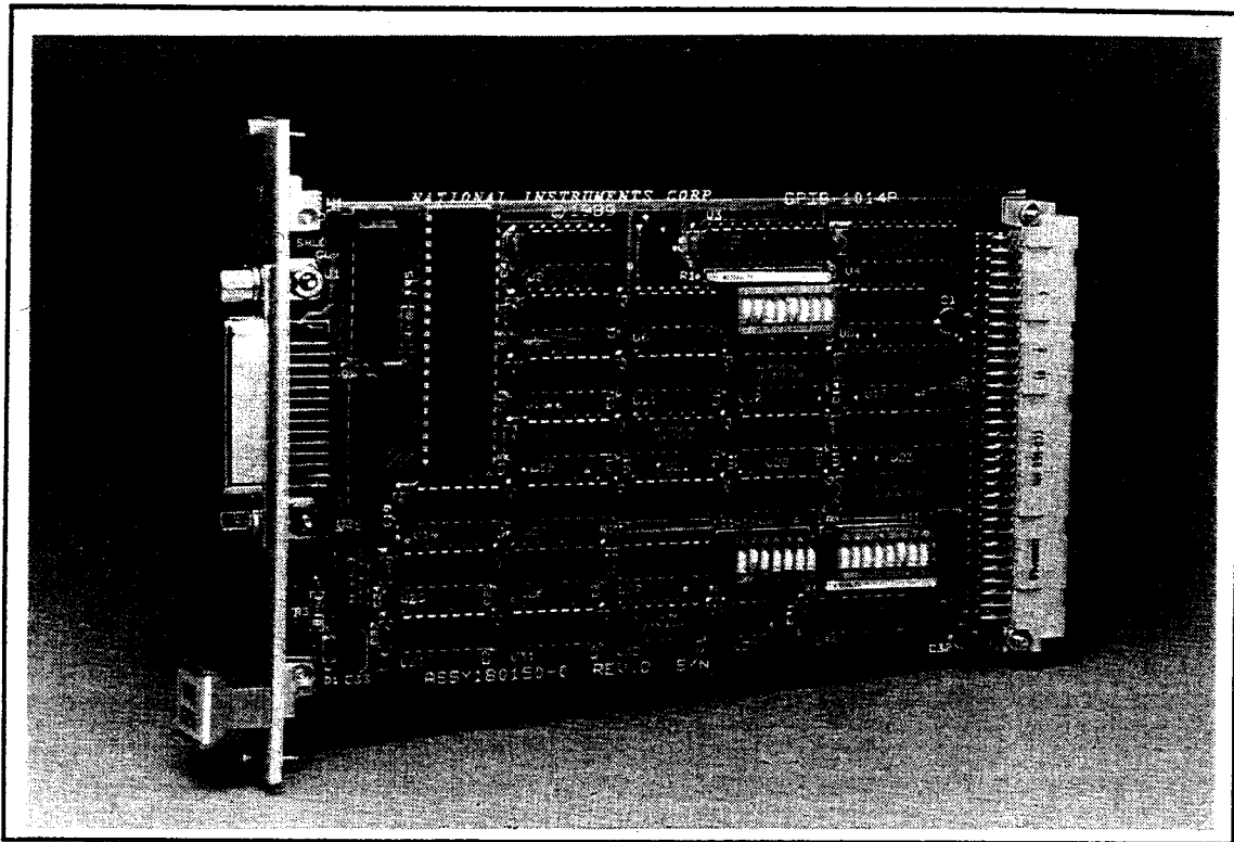
Figure 1-1. GPIB-1014P Interface Board
